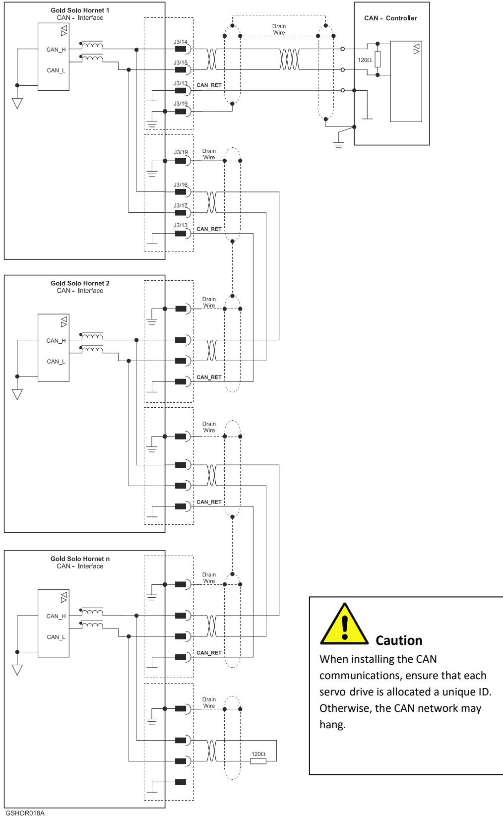
Figure 34: Gold Solo Hornet Connection Diagram – CAN
