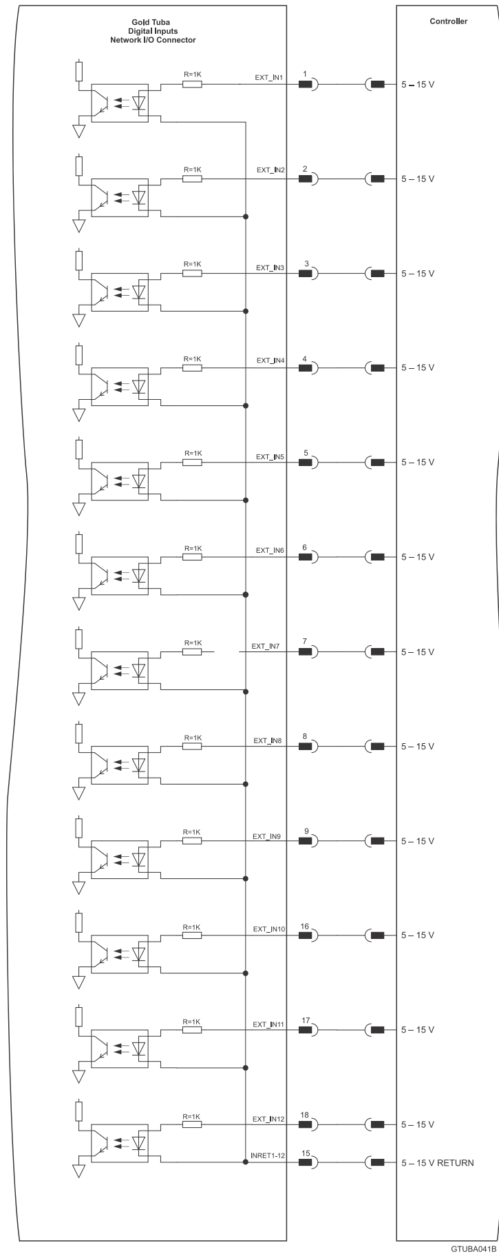
Figure 36: Network I/O Digital Input TTL Mode Connection Diagram, for G-TUBA041B
